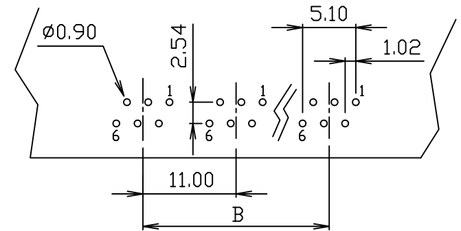
PC Board Layout Ref.
