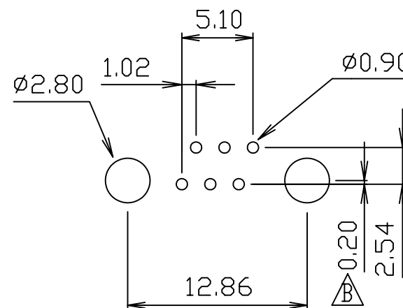
PCB LAYOUT
