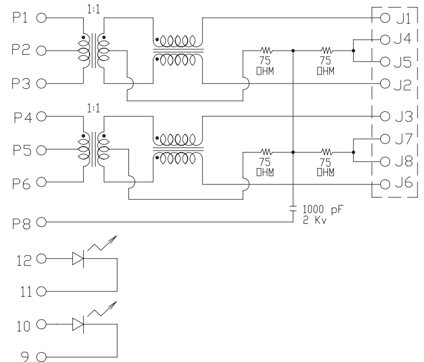
CONNECTOR SCHEMATIC
