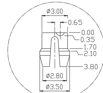
SPLIT-PEGS
