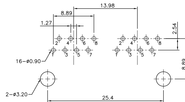
PCB LAYOUT (TOP VIEW) RECOMMENDED
