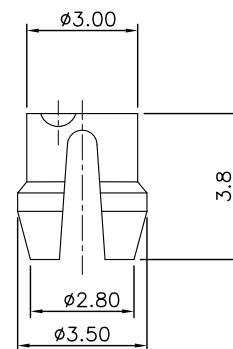
DETAIL X
