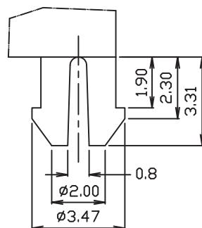
DETAIL X
