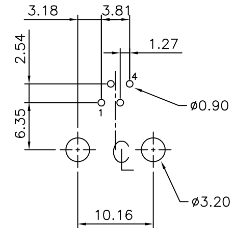
PC Board Layout Ref.
