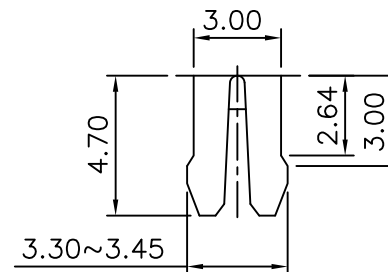
DETAIL X
