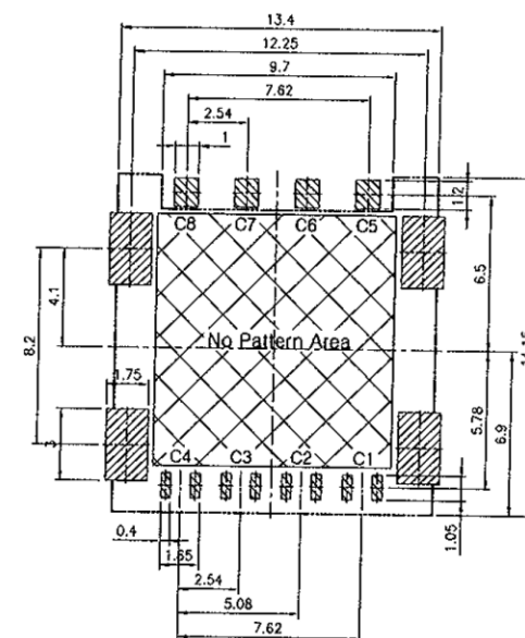
P.C.B LAYOUT (Top View) (General Tolerance \pm 0.05 )
