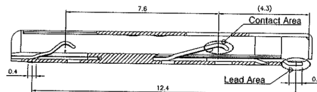
SECTION A-A' (ZOOM VIEW)
