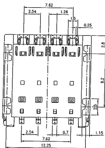
Insert Micro USIM CARD
