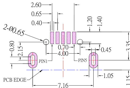
P.C.B LAYOUT MOUNTING PATTEN
