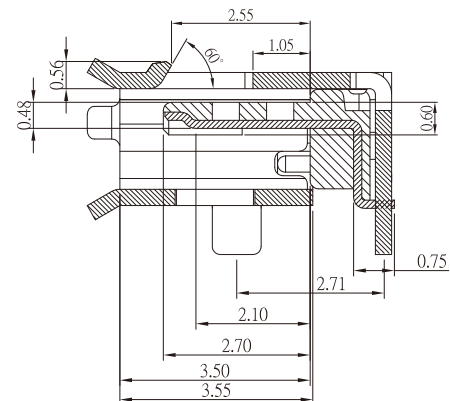
SECTION "A-A" (2:1)
