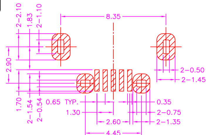
P.C.B. LAYOUT TOP VIEW \pm 0.05
