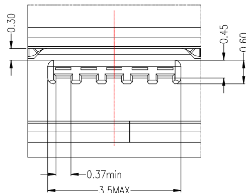
CONTACT AREA DETAIL VIEW
