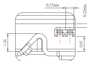
Detail C(2:1)
