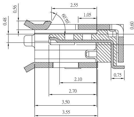
SECTION "A-A"(2:1)
