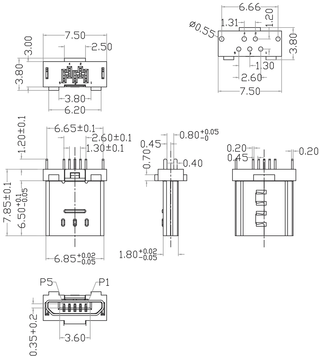
RECOMMENDED P.C.B. LAYOUT (T:0.8mm)
