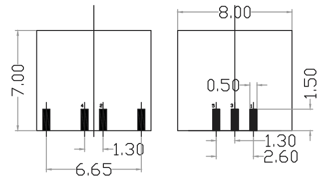
RECOMMENDED P.C.B. LAYOUT (T:0.8mm)
