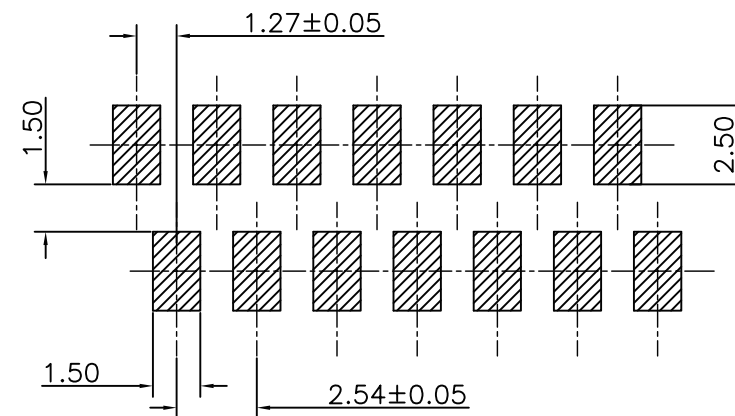
PCB Layout
