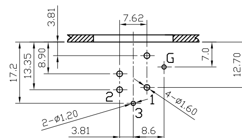
P.C.B LAYOUT( \pm 0.1 ) (BOTTOM VIEW)(SCALE 4 : 1)
