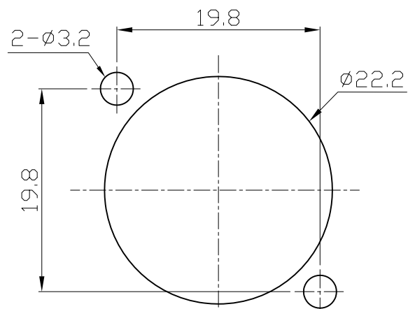
PANEL CUT OUT( \pm 0.1 ) (FRONT SIDE)
