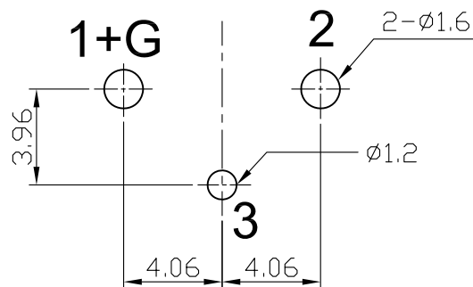
P.C.B LAYOUT (BOTTOM VIEW)(SCALE 4:1)
