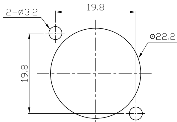
PANEL CUT OUT FRONT SIDE
