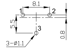
P.C.B. LAYOUT(±0.1) (BOTTOM VIEW)
