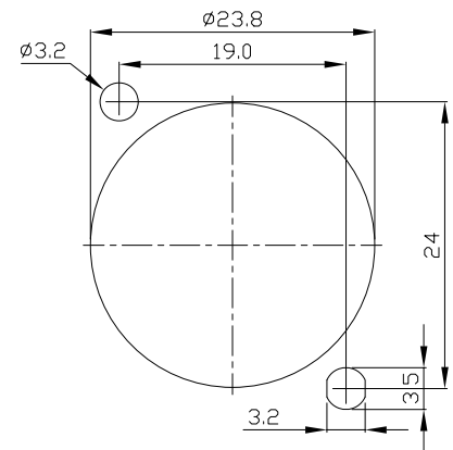
(FRONT SIDE) PANEL CUT OUT(±0.05)
