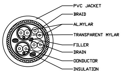
CABLE SECTION
