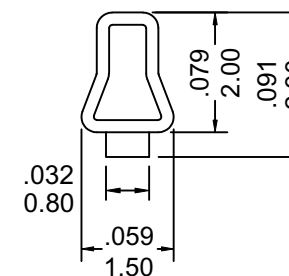
SECTION C-C
