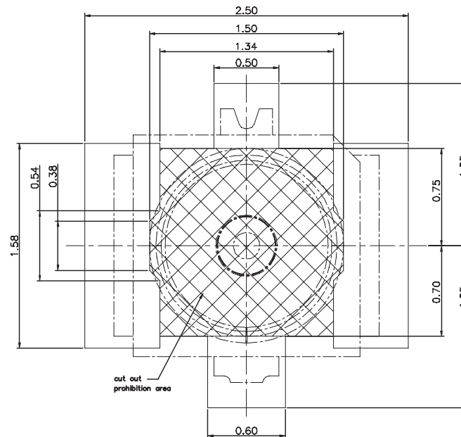
Recommended PCB Layout (General Tolerance Is \pm 0.05 )
