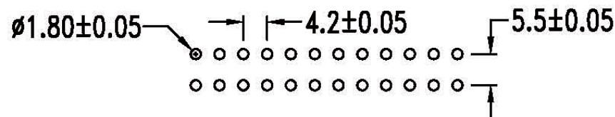
P. C. B . hole dimensions
