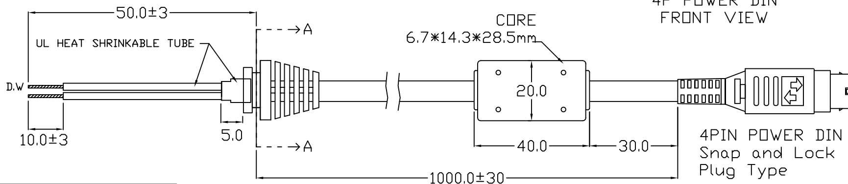
[1571#14AWG 1C+1] SECTIONAL DRAWING
