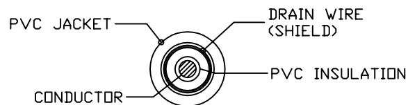
[1571#14AWG 1C+1] SECTIONAL DRAWING
