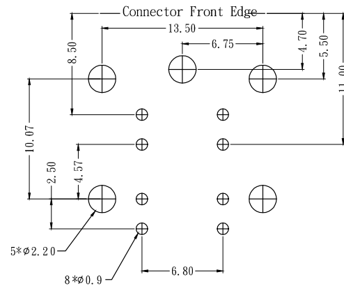
Printed Circuit Board (PCB) Layout
