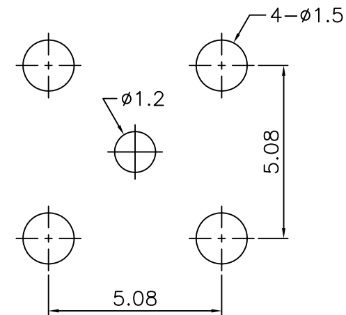
PCB MOUNTING HOLE (印刷电路板架設孔)
