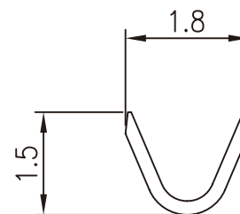
B-B SECTION
