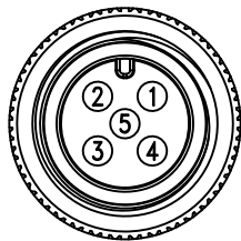
Conn.3 Pin Assignments Front View
