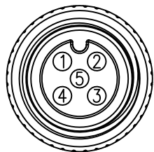
Conn.1, 2 Pin Assignments Front View
