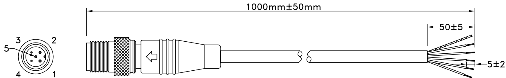
FRONT VIEW
