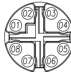
Pin Assignments
