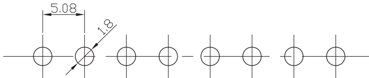
RECOMMENDED P.C.BOARD HOLE DIM.
