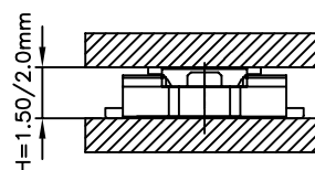
MATED DRAWING (REF) SCALE : 5 : 1
