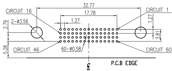
RECOMMENDED P.C.B LAYOUT INSPECTION DIMENSION(A)~(H)
