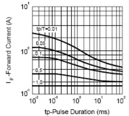
FIG.7 PULSE FORWARD CURRENT VS. PULSE DURATION
