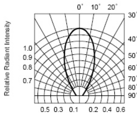
FIG.6 RADIATION DIAGRAM
