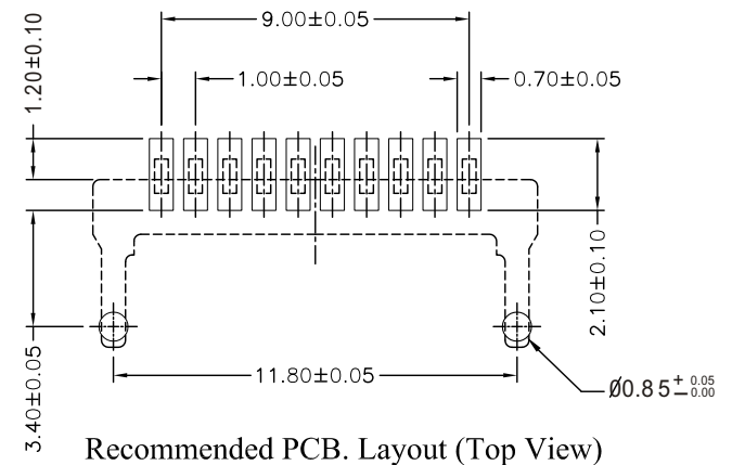
Surface Contact Layout
