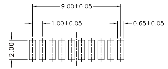
Surface Contact Layout
