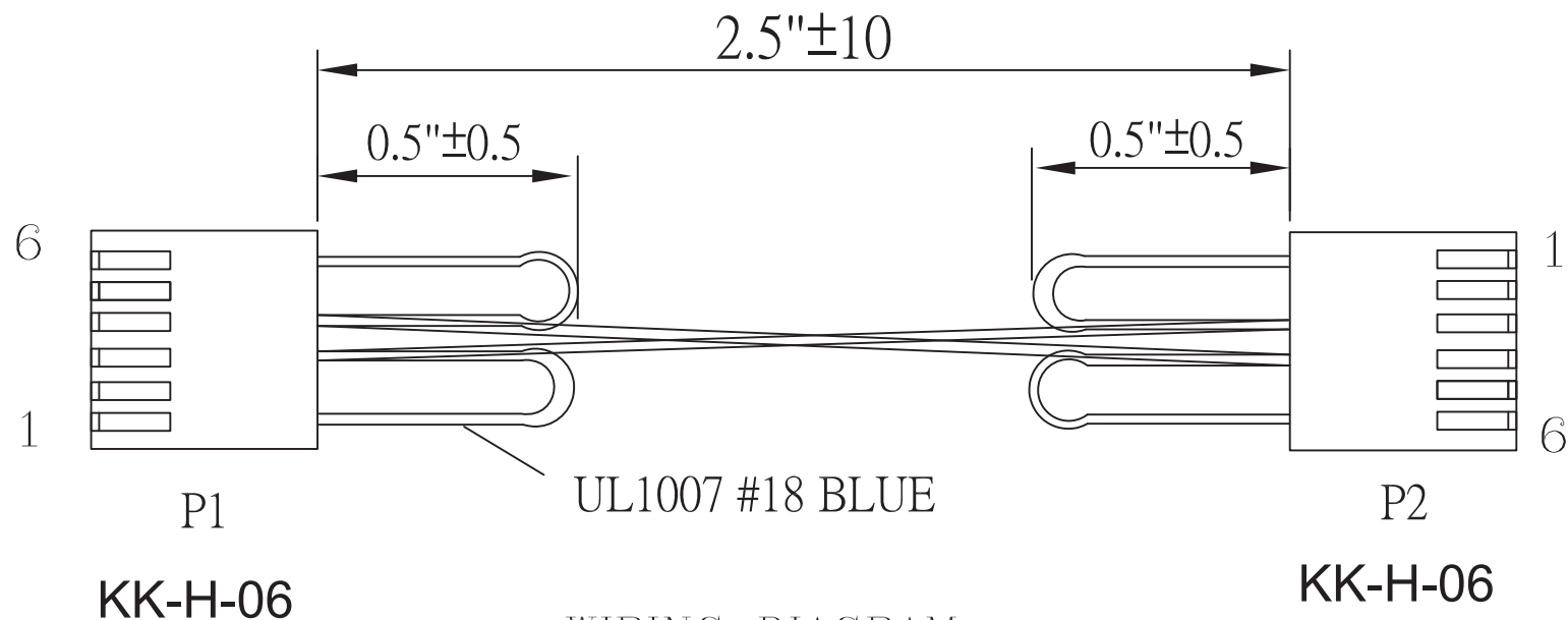
WIRING DIAGRAM
