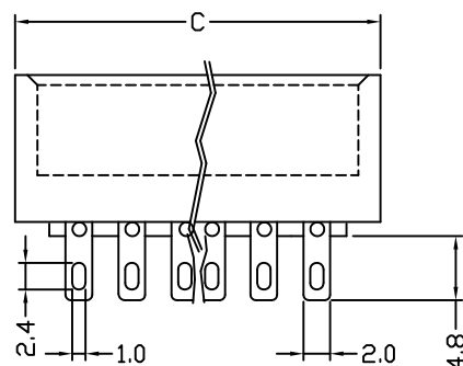
SOLDER TYPE
