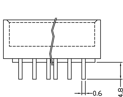
DIP TYPE
