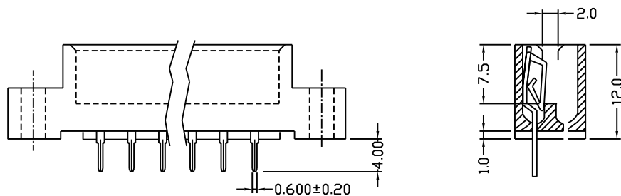
DIP TYPE
