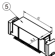
CONNECTOR VIEW
