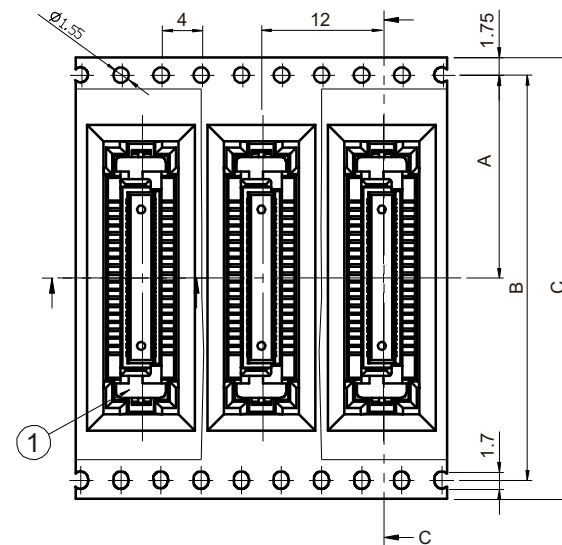
A VIEW DETAIL SCALE 2:1
