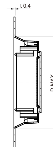
SECTION C-C SCALE 2:1
