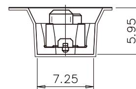
B-B Section
