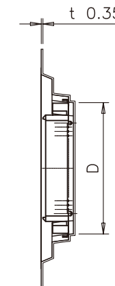
C-C Section
