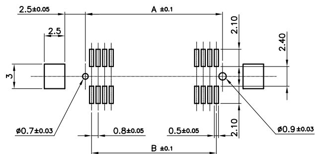
PCB. PATTERN (REF.)
