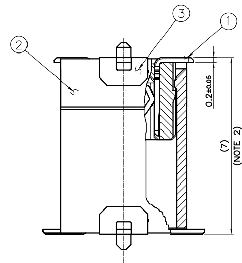
MATED CONDITION (REF.) (SCALE 9:1)
