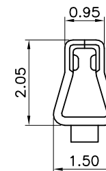
Section C-C
