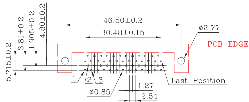
PCB Layout (A)
