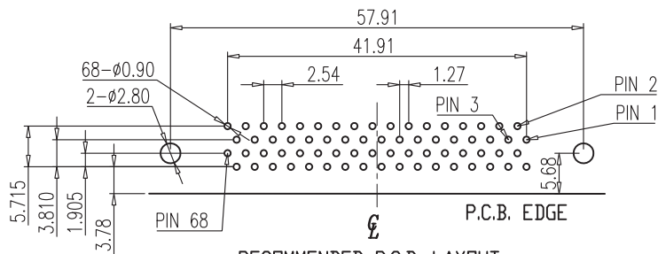
RECOMMENDED P.C.B. LAYOUT INSPECTION DIMENSION:(A)~(J)
