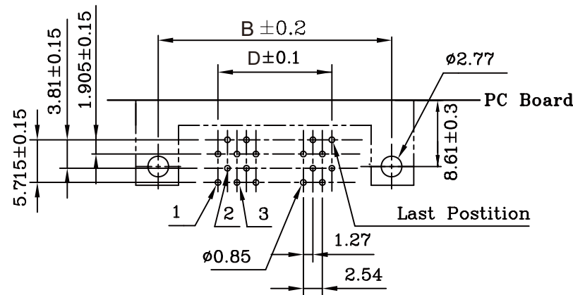
PCB LAYOUT
