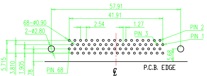
RECOMMENDED P.C.B. LAYOUT INSPECTION DIMENSION:(A)~(J)
