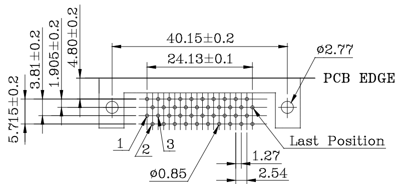
PCB Layout (B)
