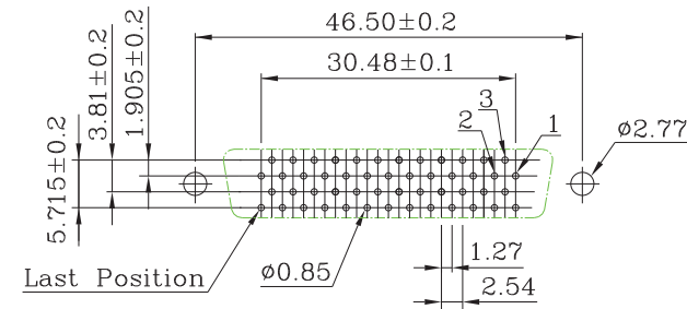
PCB Layout (A2)
