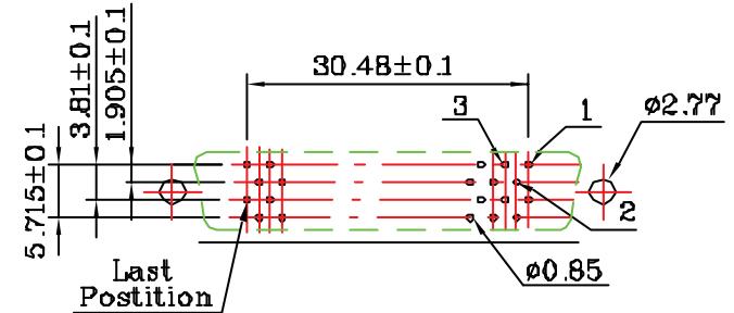
1N: Standard P.C.Board Hole Pattern
