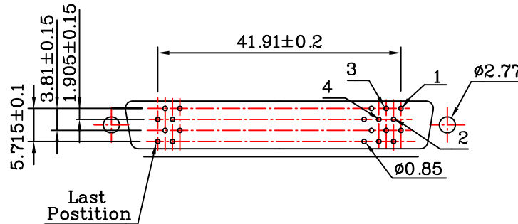
L1:Reveres PCB LAYOUT
