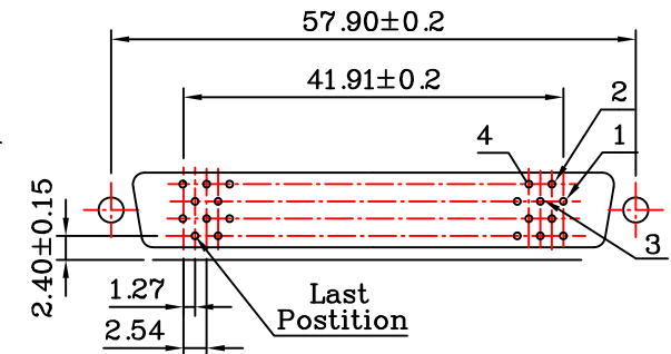
L2:Standard PCB LAYOUT
